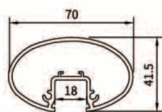
扶手面管 TOP RAIL (01-142) (2001-10)
