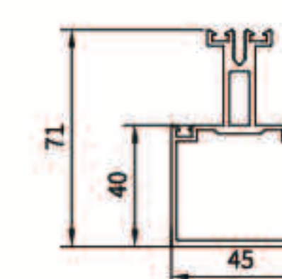
副梁 CURTAIN WALL FRAME-HORIZONTAL
