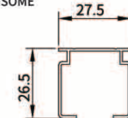
压条 TRANSOME
