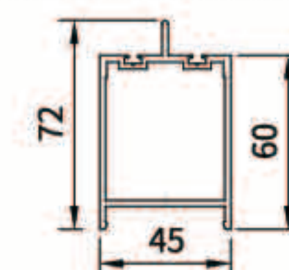
副梁 CURTAIN WALL FRAME-HORIZONTAL
